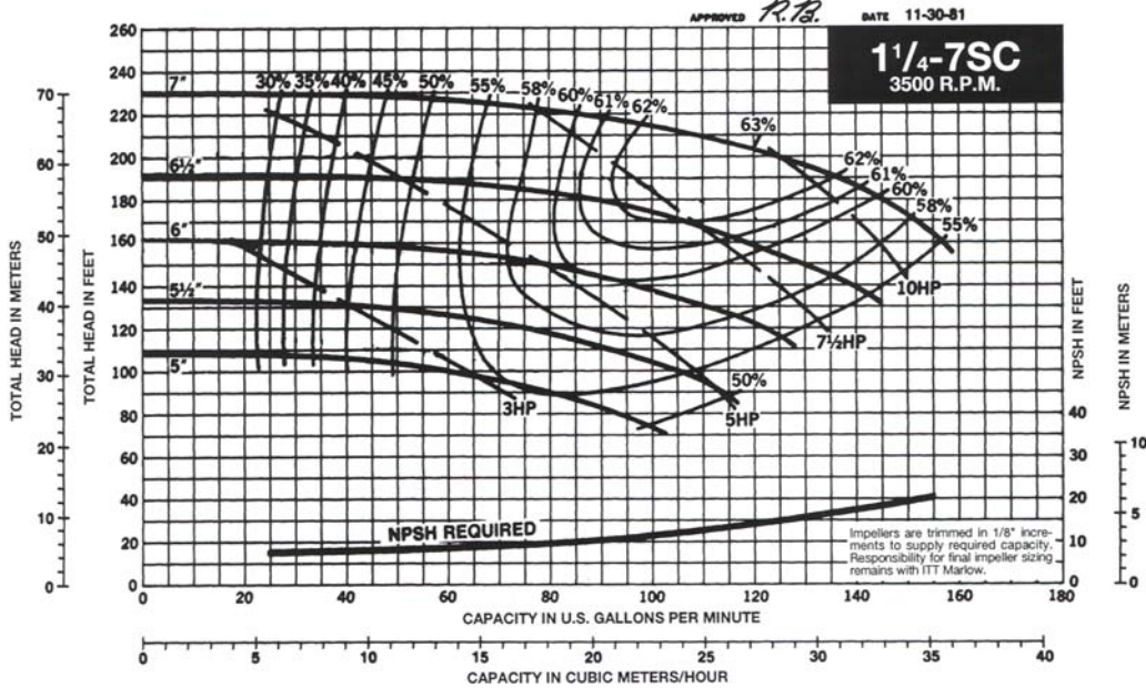
PERFORMANCE CHARACTERISTIC CURVE
